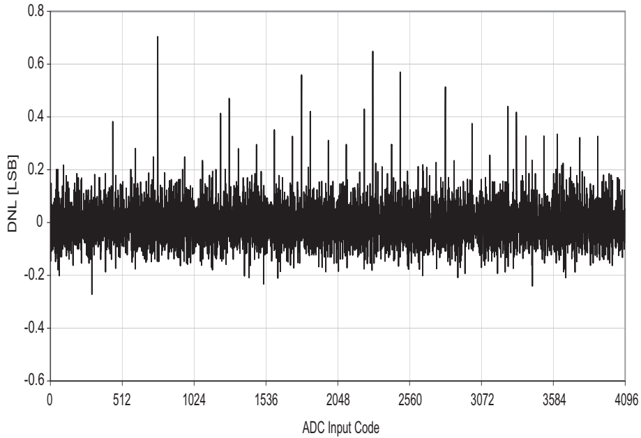
Figure 37-293. DNL error vs. input code
